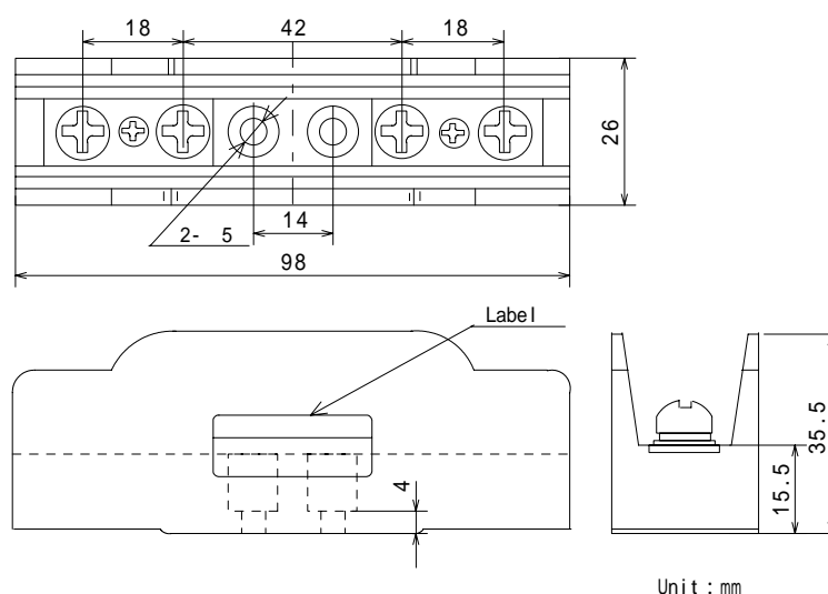
For 200A fuse holder dimension drawing
