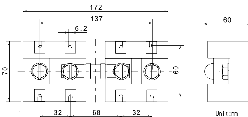
For 200A fuse holder dimension drawing
