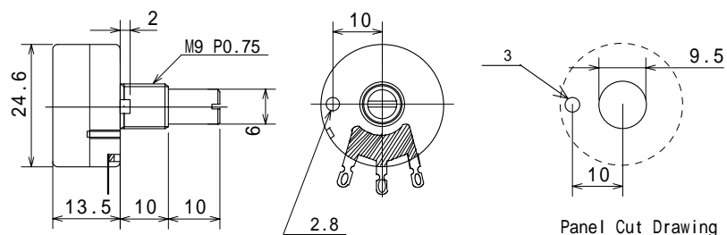
External Variable Resistor (Resistance : 10k Characteristic : B) Unit : mm
