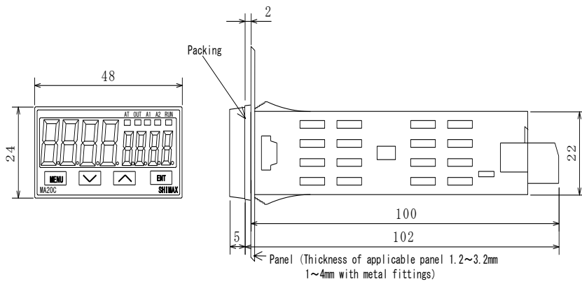
MA20C panel cutout (unit : mm)
